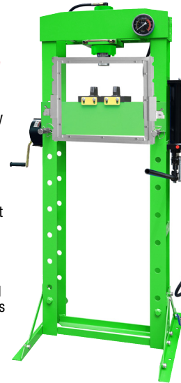
Adjustable Hydraulic Cylinder
