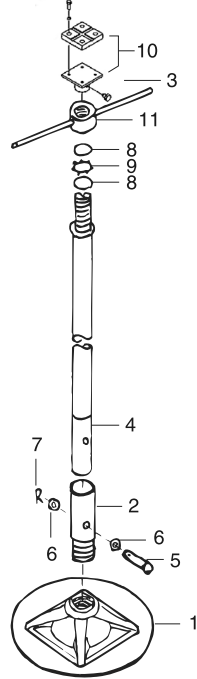
Parts Diagram
